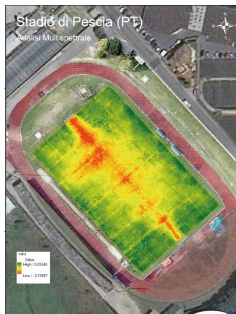
Fig. 5 - Aerial multispectral images.
